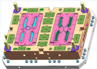
平行注射双色模 Parallel two-colour mould
