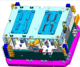
旋转托芯双色模 Rotary-core two-colour mould
