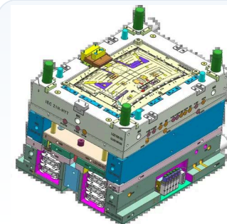
台式电脑后盖 Desktop PC rear cover
