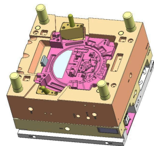
扫地机面壳 Robot vacuum top shell
